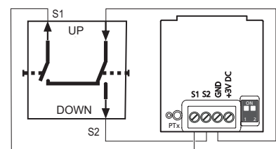
Motor switch connection
